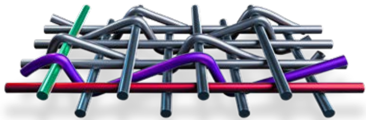
The unique straight-warp construction of the UsFlex carcass
